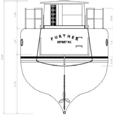
REAR ELEVATION
