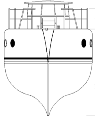
FRONT ELEVATION
